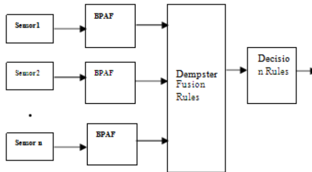
Figure 1: Architecture
