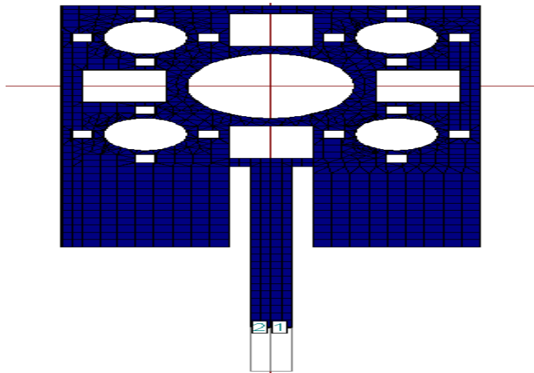
Figure 8. Geometry of iteration III for proposed antenna. Big square=4*4mm (7,0),small square=1*1mm(6,9)
