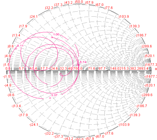
Figure 7. Input impedance loci using smith chart of iteration II
