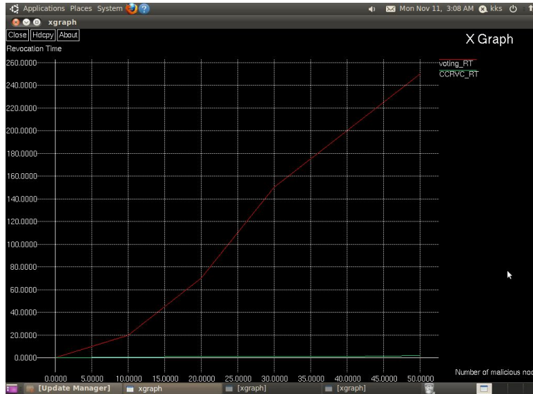
Fig 4c Revocation time graph
