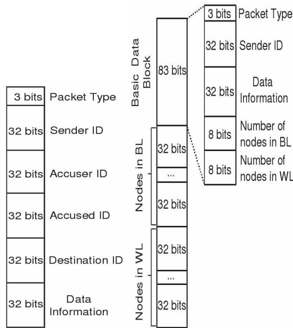
Fig. 2. Control packets.
