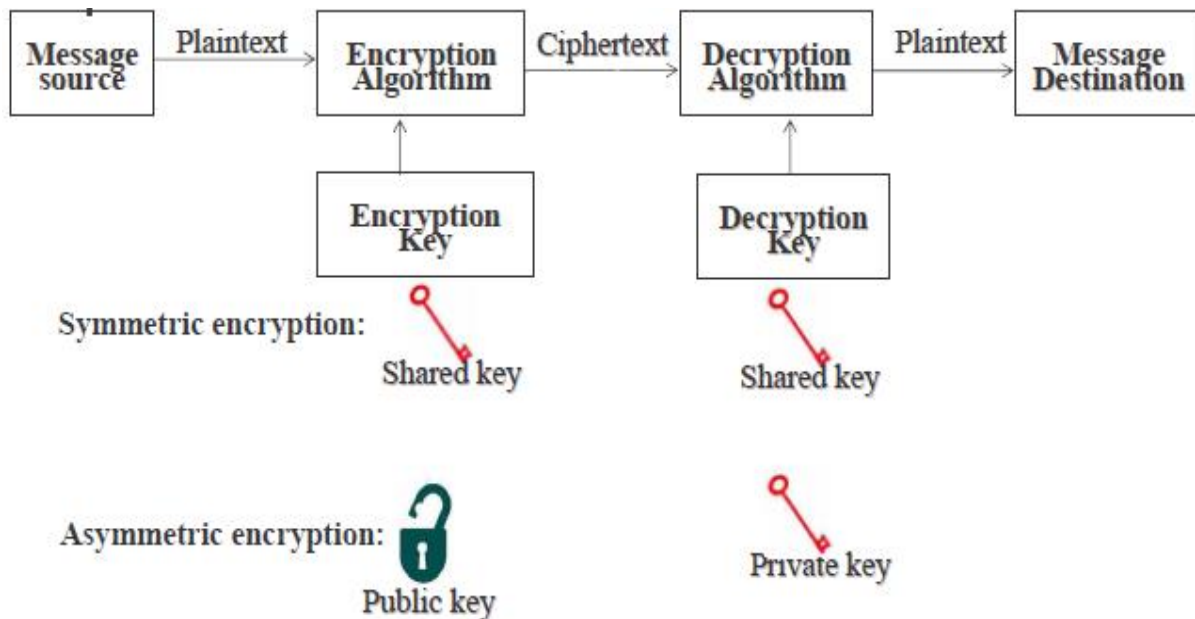
Fig 2: Cryptography
