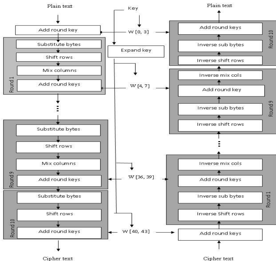
Fig. 1: Encryption and decryption in AES
