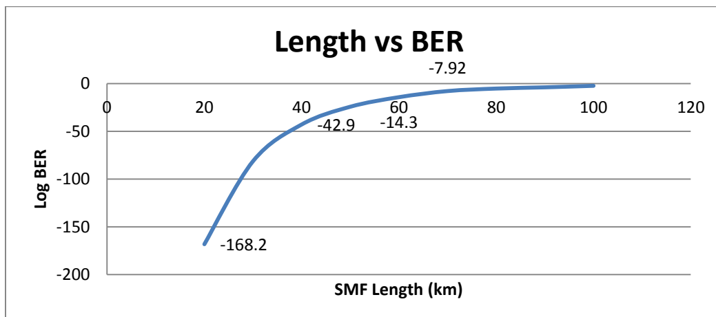
Graph 1: Length of SMF v/s BER without FBG
