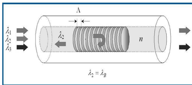
Figure 1: Principle operation of FBG
