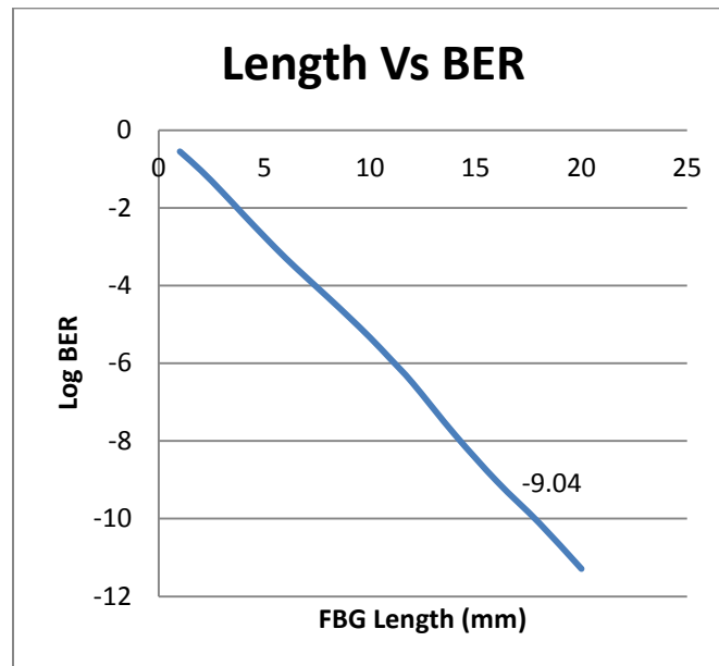
Graph 2: Length of FBG v/s BER
