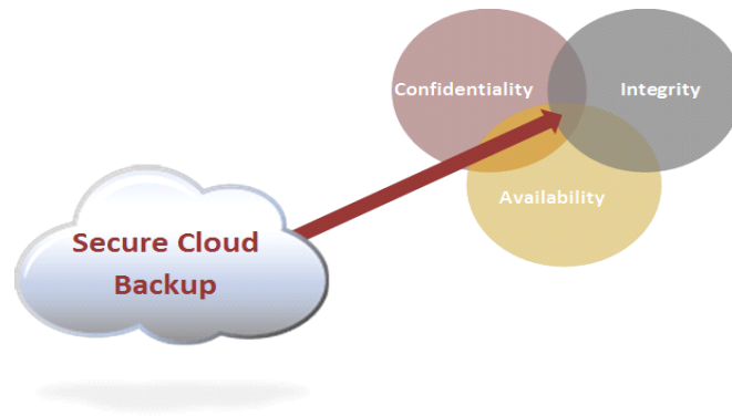
Fig. 1 cloud computing
