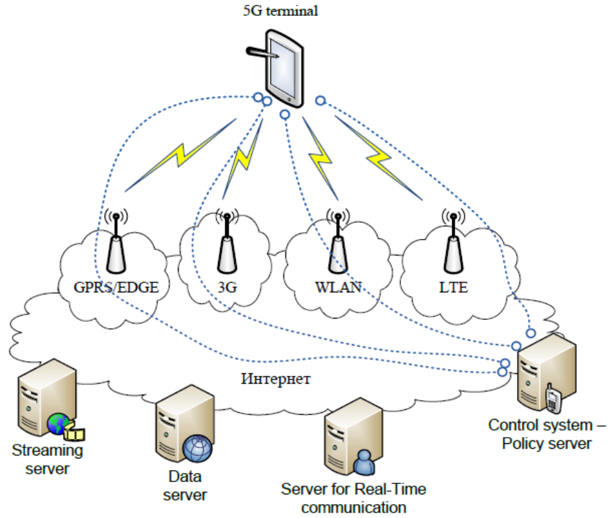
Fig : 5G Mobile Network Architecture
