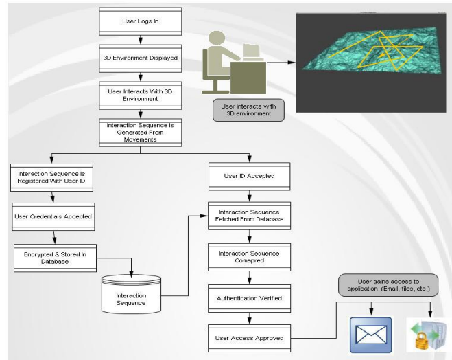
Fig.4 working of 3d password scheme [5]
