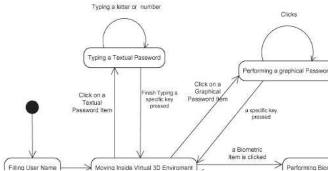
.Fig.3 state diagram of creating 3D password [1] [6] [7]
