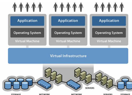
fig3: Virtualization mechanism
