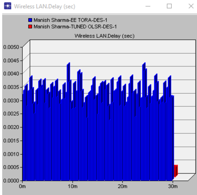
Figure 2 OLSR and TORA Delay
