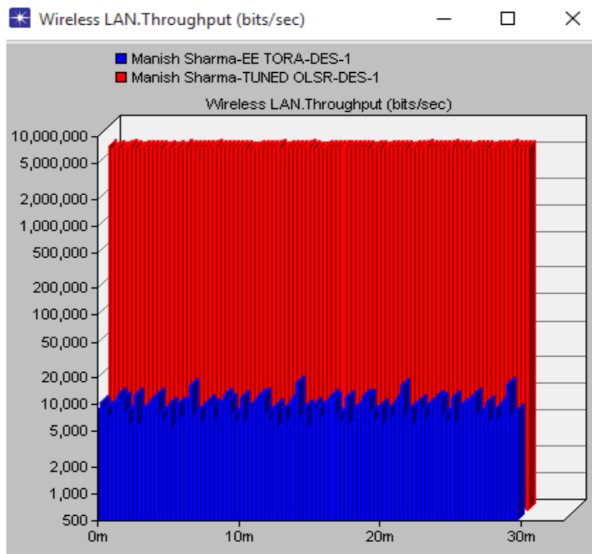
Figure 5 OLSR and TORA Throughput
