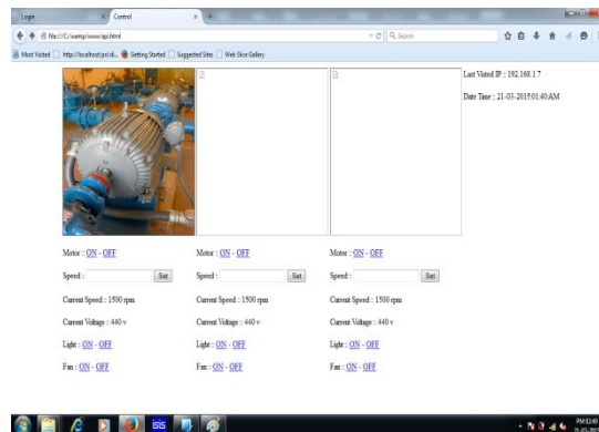
Fig 5 Control page
