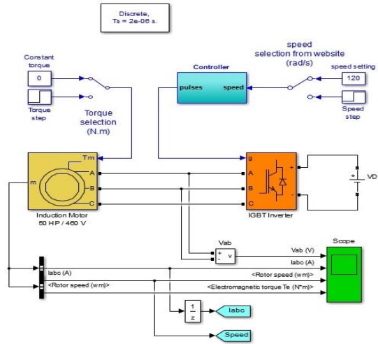
Fig 2. Simulation block
