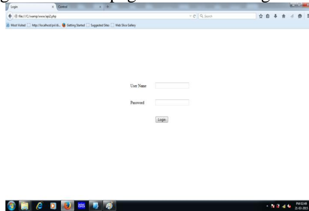
Fig 4. Login page
