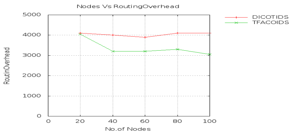
Fig 13 Nodes Vs Overhead
