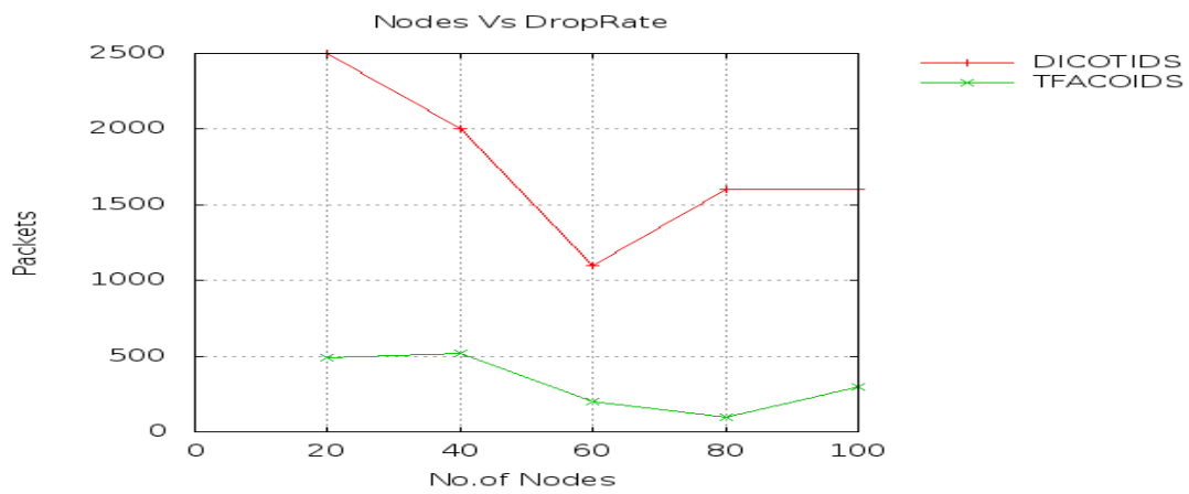
Fig 13 Nodes Vs Drop Rate
