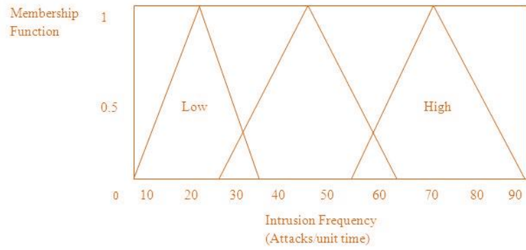
Fig 2: Membership Function Of Intrusion Frequency
