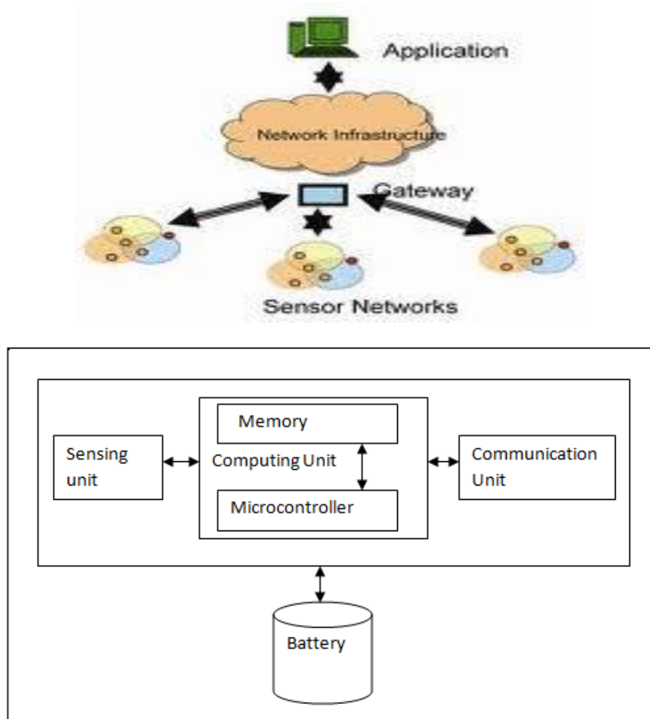
Fig. 1 Schematic of a Wireless Sensor Network Architecture
