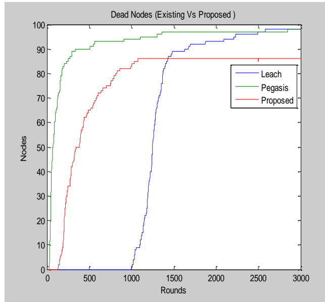
Fig. 3 Comparative Analysis (LEACH Vs Existing Vs Proposed) Dead Nodes
