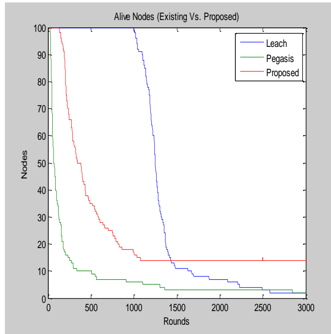
Fig. 4 Comparative Analysis (LEACH Vs Existing Vs Proposed ) Alive Nodes
