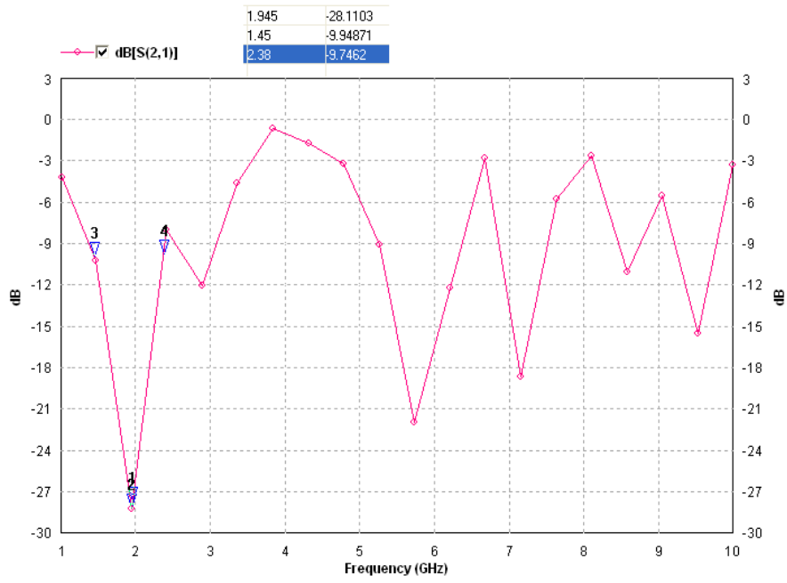
Figure 3. Return loss vs. Frequency curve of iteration I for proposed antenna
