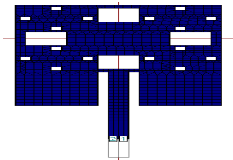
Figure 2. Geometry of iteration 1 with t=1.524 , Permittivity=4.4 and grid size=.025 , l=20 , w=20 , feed length=20mm, feed width=2mm. big square= 4*4,small square=1mm.
