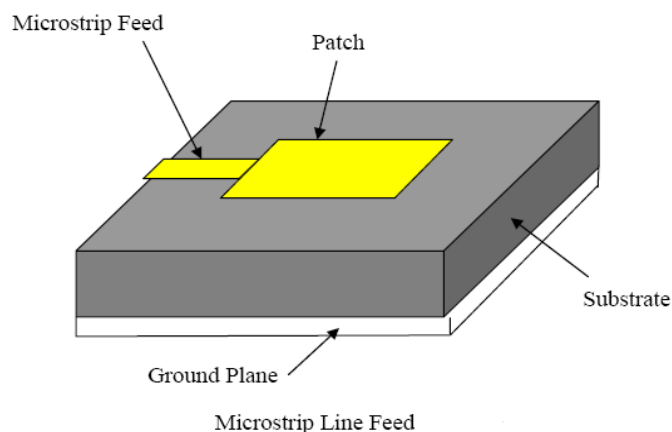
Figure 1: Microstrip line feed
