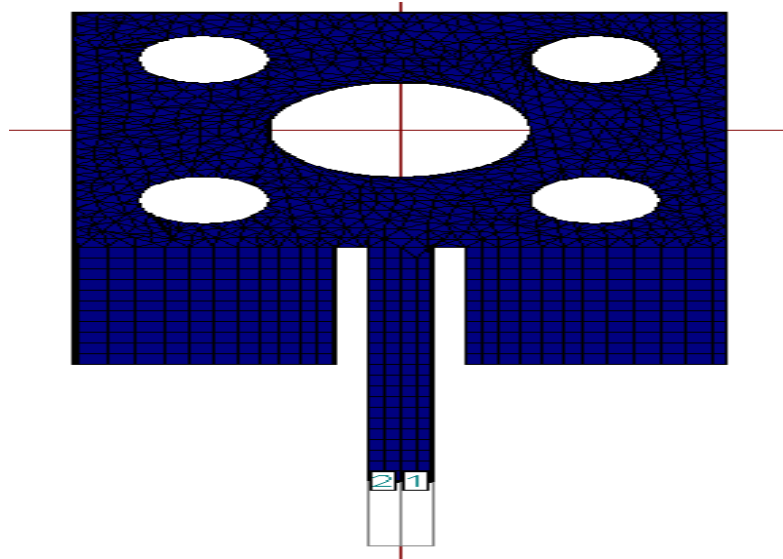
Figure 5. Geometry of iteration II for proposed antenna. Big circle=4mm(0,0),small circle=2mm,radius(6,6)
