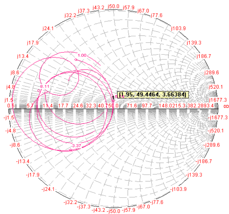
Figure 4. Input impedance loci using smith chart of iteration I
