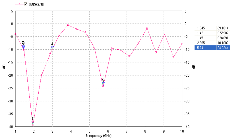
Figure 9. Return loss vs. frequency of iteration III for proposed antenna
