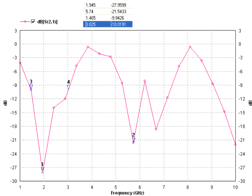
Figure 6. Return loss vs. Frequency curve of iteration I for proposed antenna
