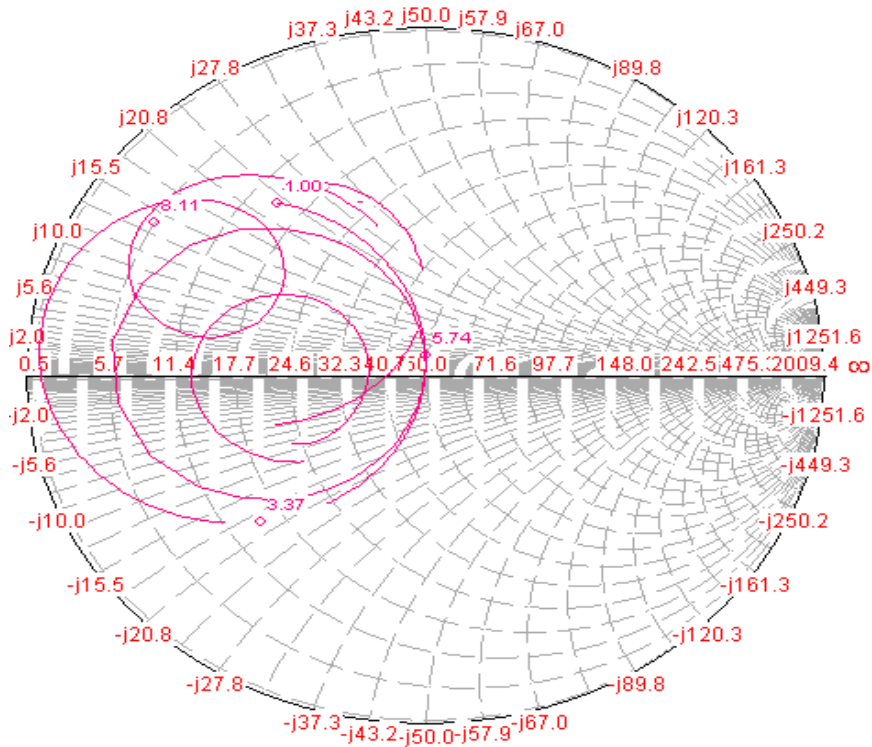
Figure 10. Input impedance loci using smith chart for iteration III
