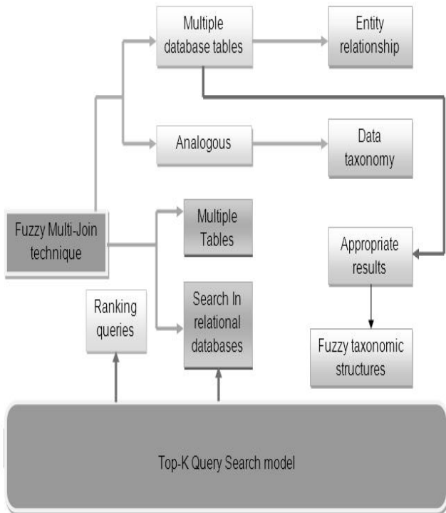
Fig. 1 Architecture Diagram of Fuzzy Multi-Join and Top-K Query Model for Search-As-You-Type in Multiple Tables
