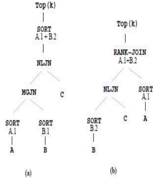
Fig.4 Alternative plans for Query Q1
