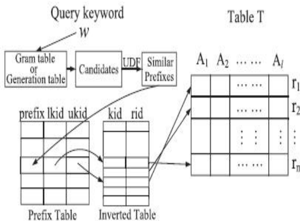
Fig.2 Using the q-gram table and the neighborhood generation table to Support fuzzy search.
