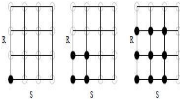
Fig. 3 Three steps in Ripple Join
