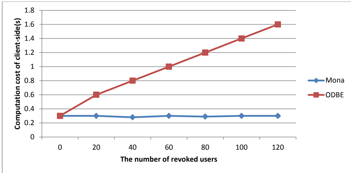
Figure 6 – Computational cost for file generation (10 MB)
