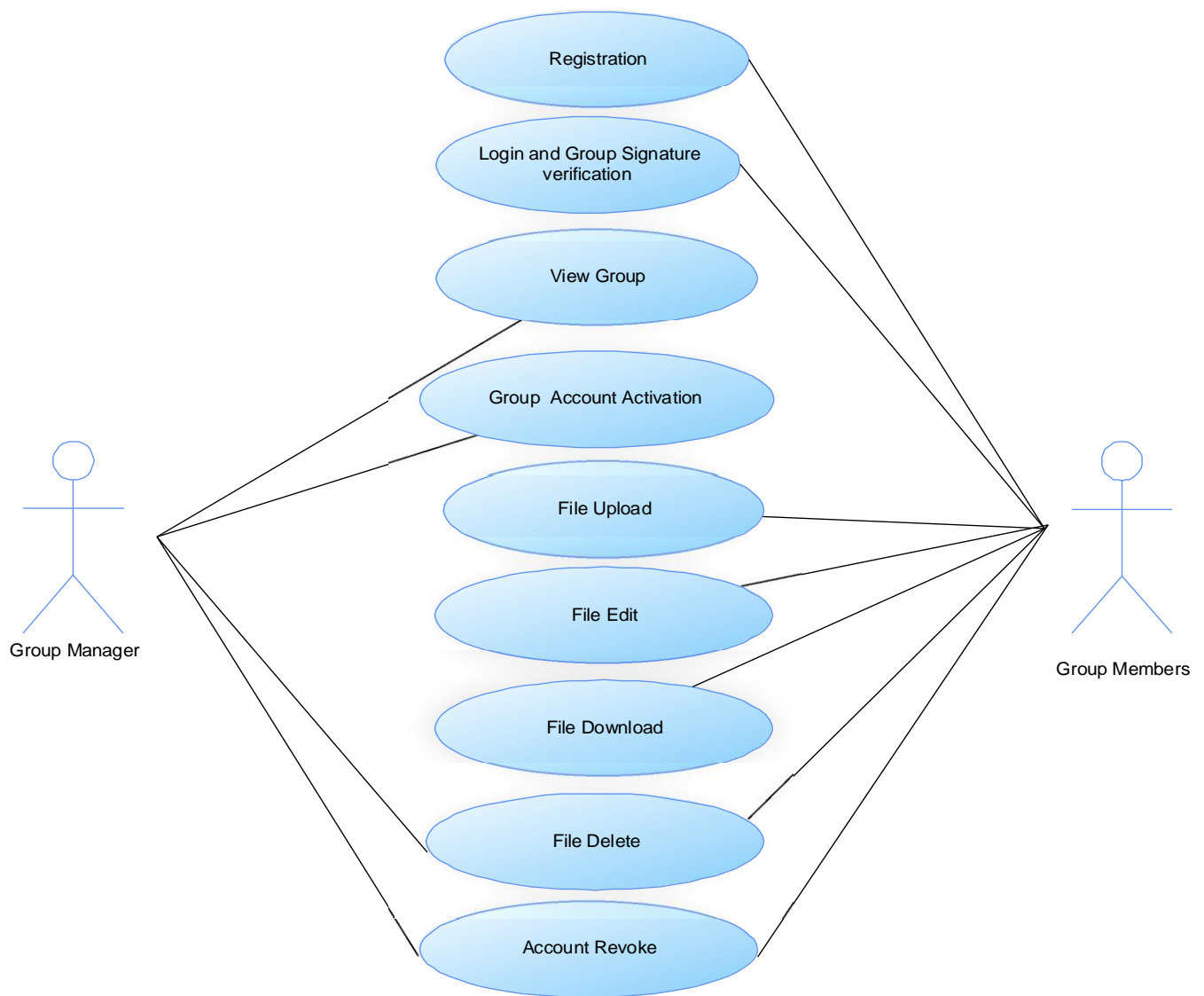
Figure 3 – USE CASE diagram showing important functionalities of the system
