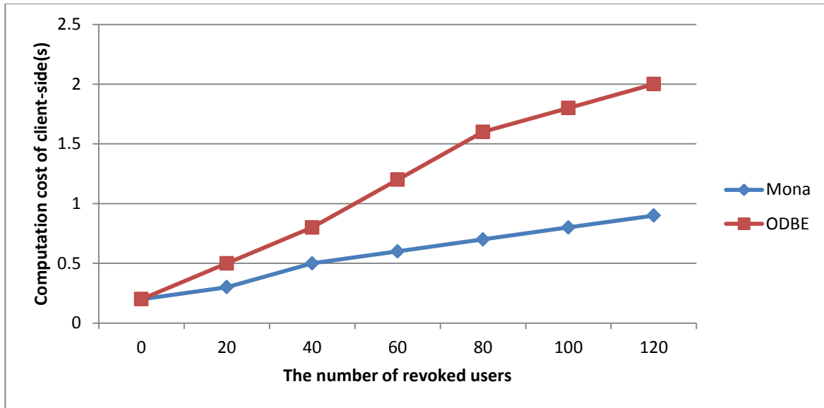
Figure 8 – Computational cost for file accessing (10 MB)
