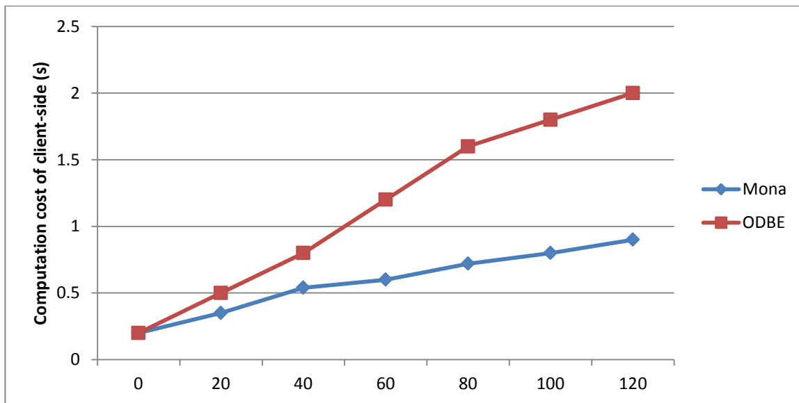
Figure 8 – Computational cost for file accessing (100 MB)
