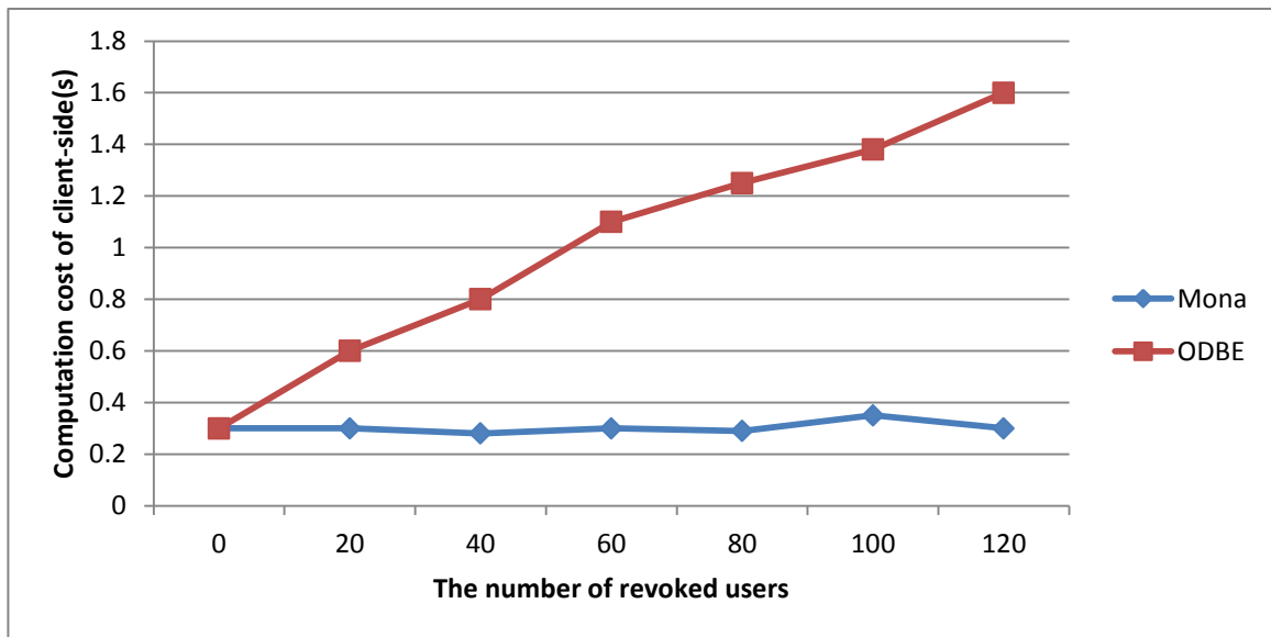
Figure 7 – Computational cost for file generation (100 MB)
