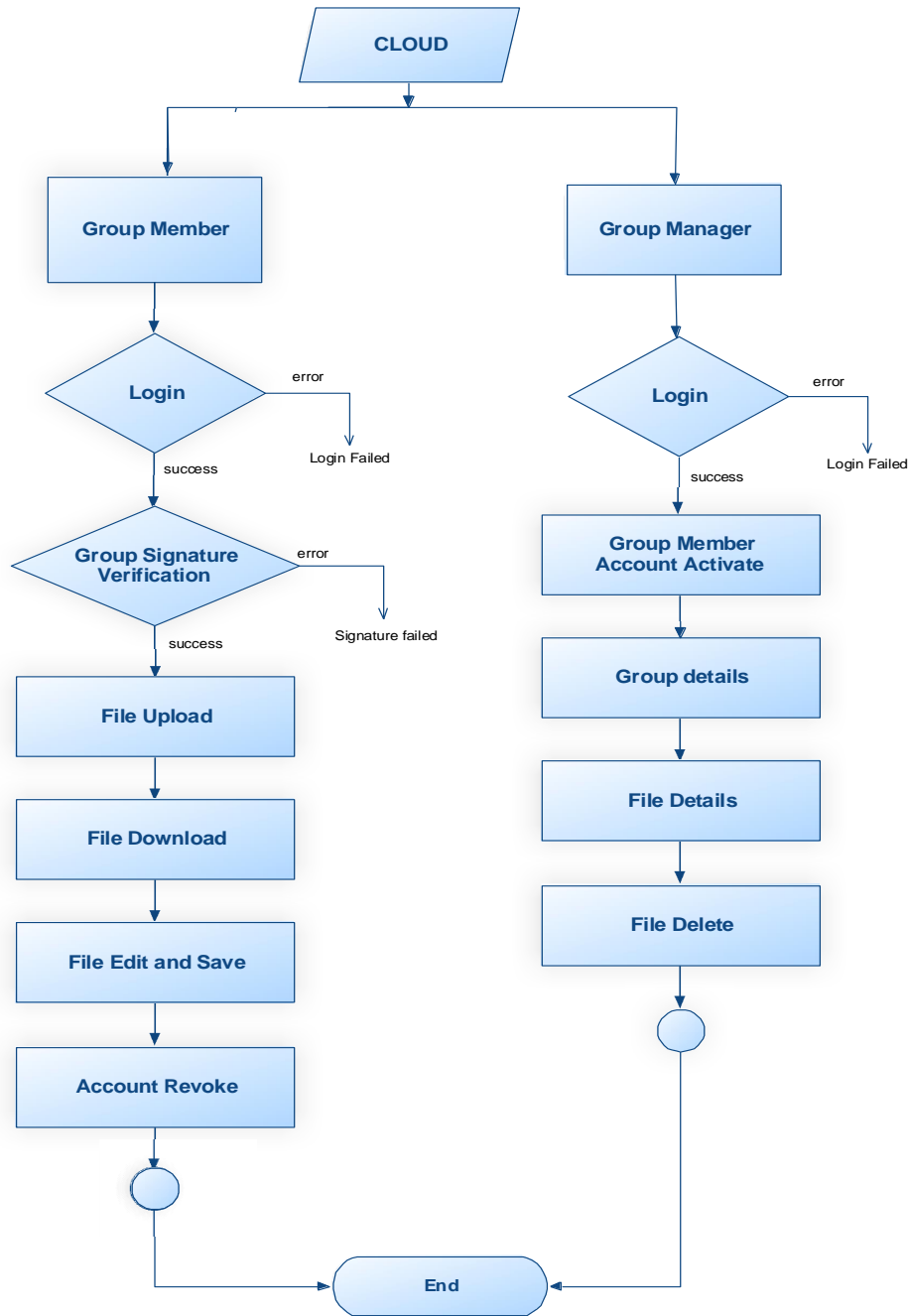
Figure 2 – The flow of activities of group manager and group member
