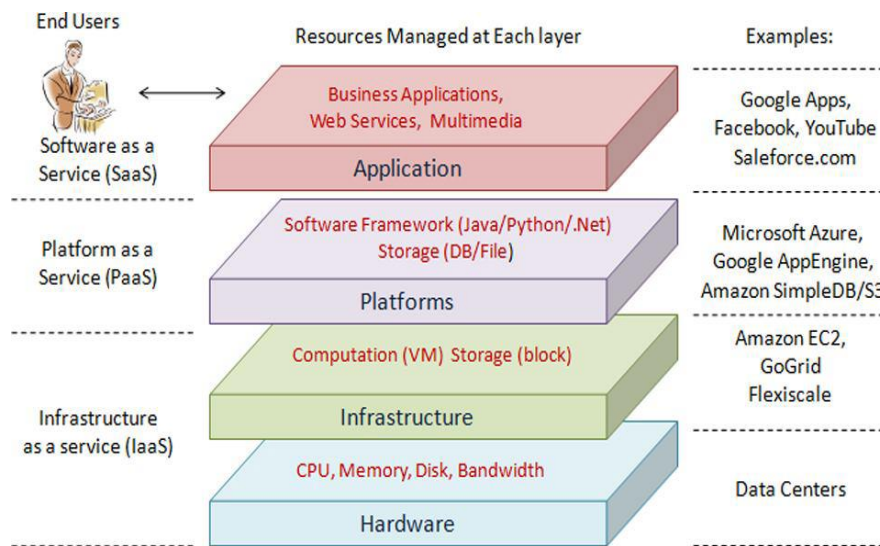
Fig. 1: Layered Model of Cloud Computing
