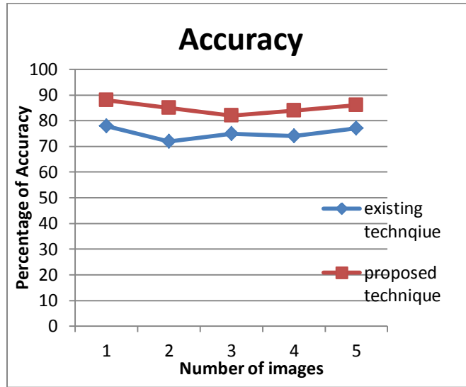
Fig 2: Accuracy Comparison
