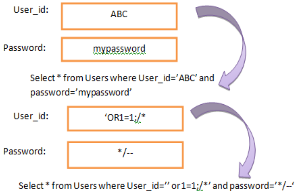
Fig. 1 SQL Injection
