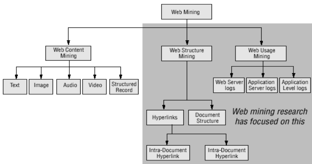
Fig 1. Web Mining Taxonomy
