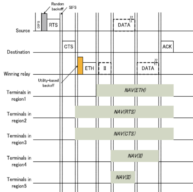
Fig. 3. NAV setting for DEL-CMAC.
