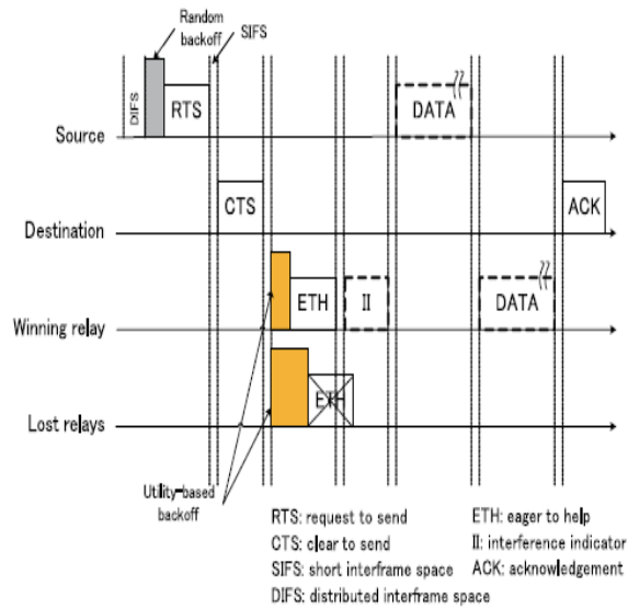
Fig. 2. The frame exchanging process of DEL-CMAC.
