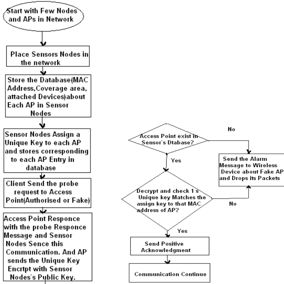
Figure 3: Flow Chart of Proposed Technique
