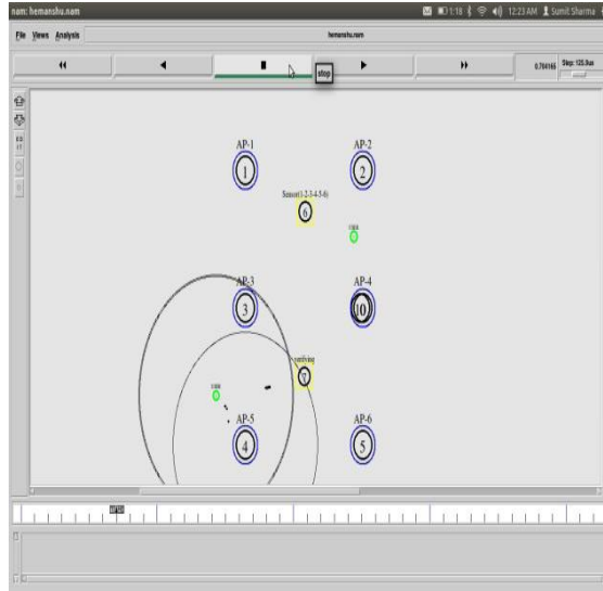
Figure 6: Verifying the access point identity by sensor node.
