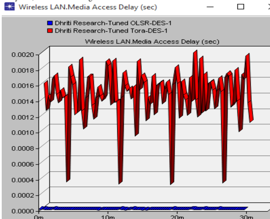
Figure 3 OLSR and TORA Medium Access Delay
