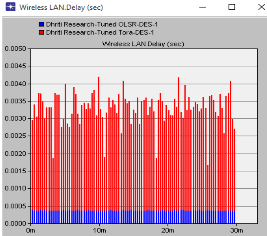
Figure 2 OLSR and TORA Delay
