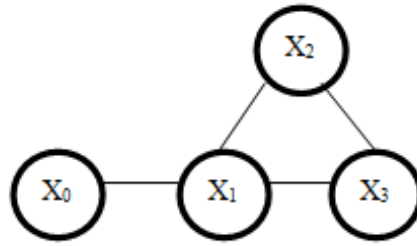
Fig 1: MRF Model
