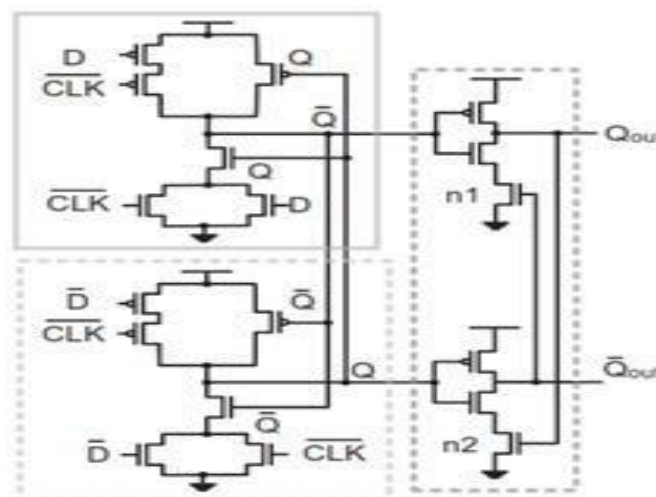
Fig 2:Proposed MRF Latch
