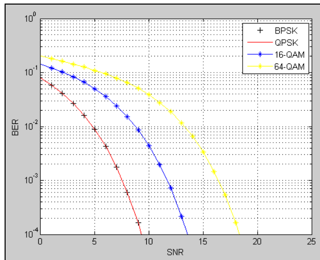
Fig. 6: BER vs SNR for Basic OFDM model (with cyclic prefix)
