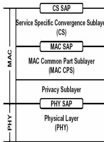
Fig. 1: WiMAX physical and MAC layer architecture
