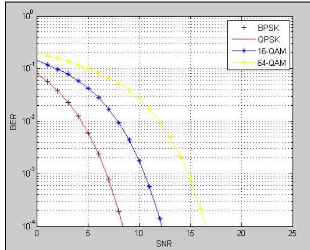
Fig. 5: BER vs SNR for Basic OFDM model (without cyclic prefix)
