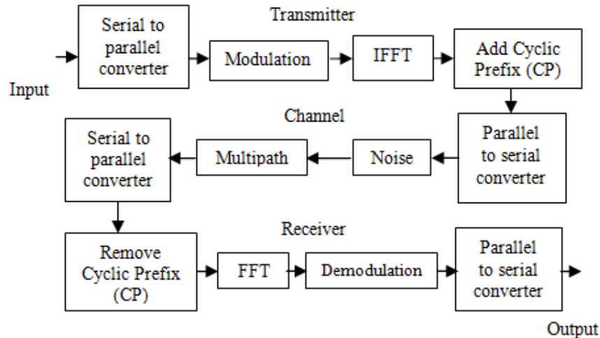
Fig. 4: OFDM Model with Cyclic Prefix
