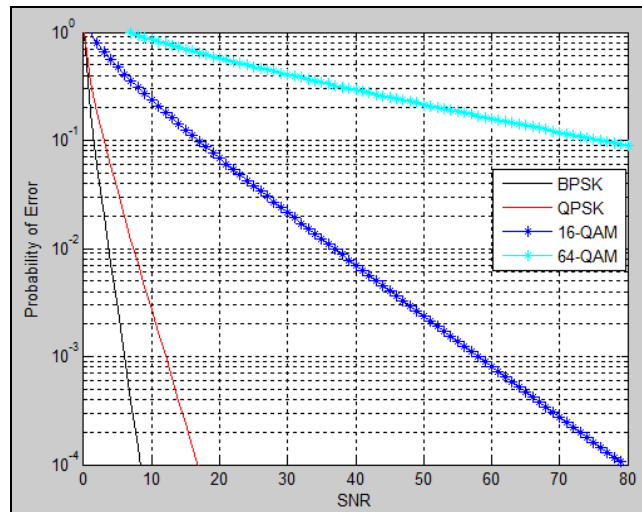
Fig. 7: Probability of error
