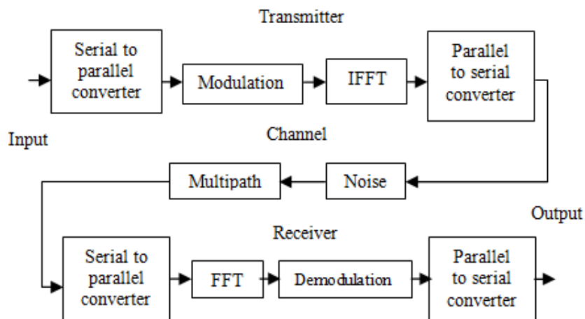
Fig. 3: OFDM Basic Model
