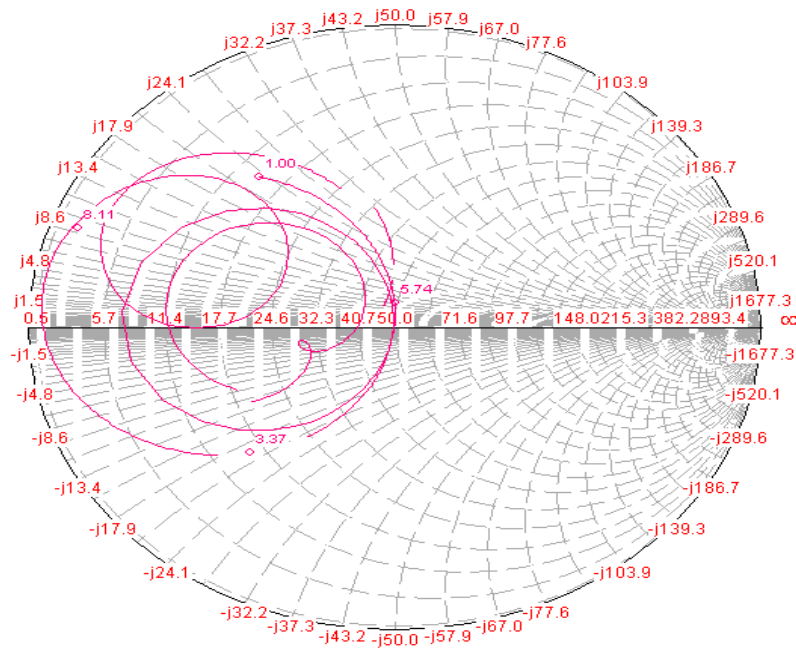
Figure 7. Input impedance loci using smith chart of iteration II
