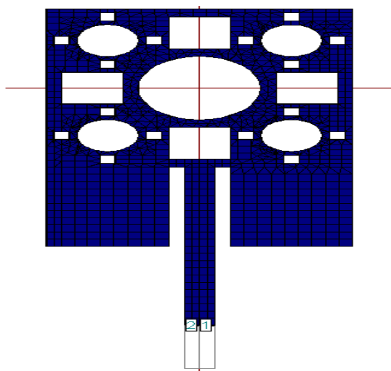
Figure 8. Geometry of iteration III for proposed antenna. Big square=4*4mm (7,0),small square=1*1mm(6,9)
