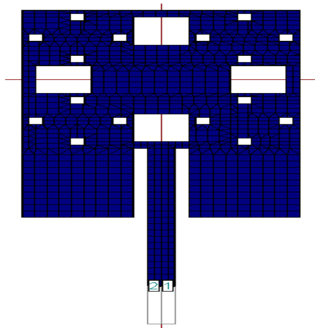
Figure 2. Geometry of iteration 1 with t=1.524 , Permittivity=4.4 and grid size=.025 , l=20 , w=20 , feed length=20mm, feed width=2mm. big square= 4*4 ,small square=1mm.
