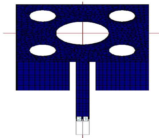
Figure 5. Geometry of iteration II for proposed antenna. Big circle=4mm(0,0),small circle=2mm,radius(6,6)
