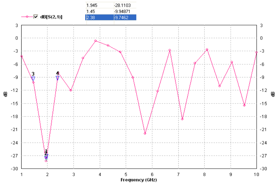
Figure 3. Return loss vs. Frequency curve of iteration I for proposed antenna
