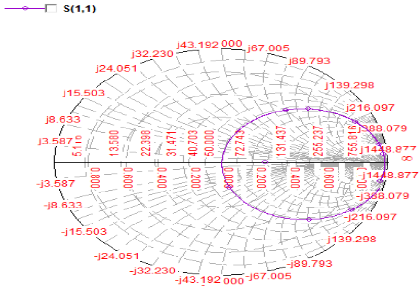
Figure 4. Input impedance loci using smith chart for iteration I
