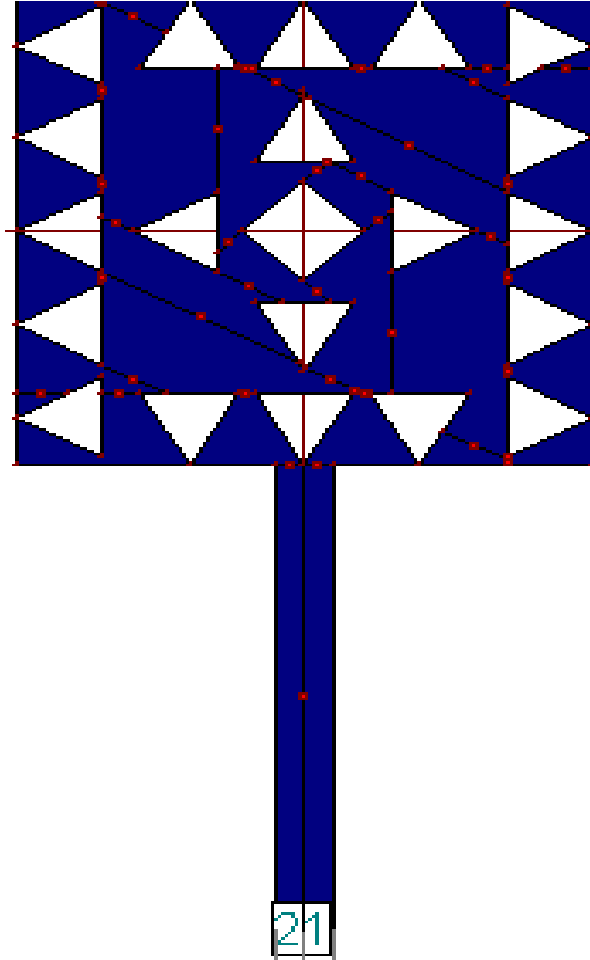
Figure 2. Geometry of iteration 1 with t=1.524 , Permittivity=4.4 and grid size=.025 , l=20 , w=20 , feed length=20mm, feed width=2mm
