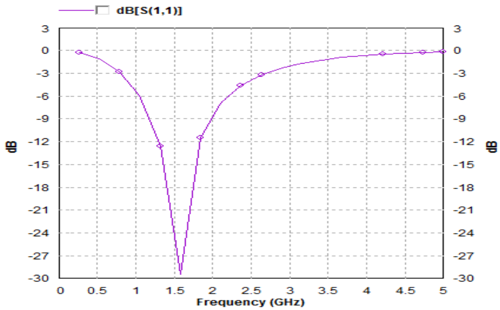
Figure 3. Return loss vs. frequency of iteration I for proposed antenna
